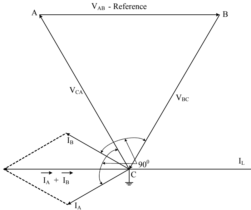
Figure 5-8—Voltages and ground fault currents in resonant-grounded system
