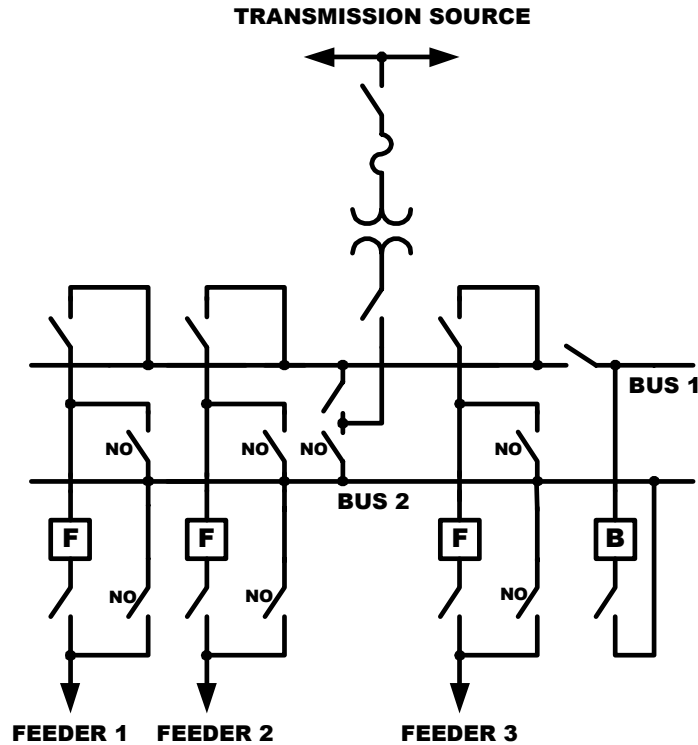
Figure 5-17—Dual-operation bus
