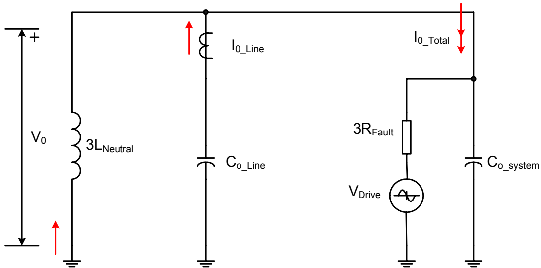
Figure 8-12—Zero-sequence network diagram for a reverse fault
