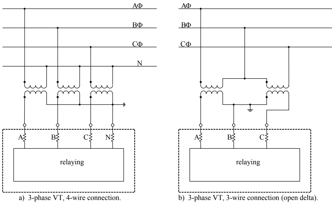
Figure 5-31—VT connections
