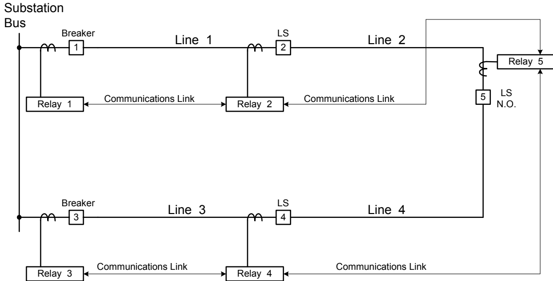
Figure 8-6—Communications-enhanced trip and restore scheme on a looped-radial distribution system
